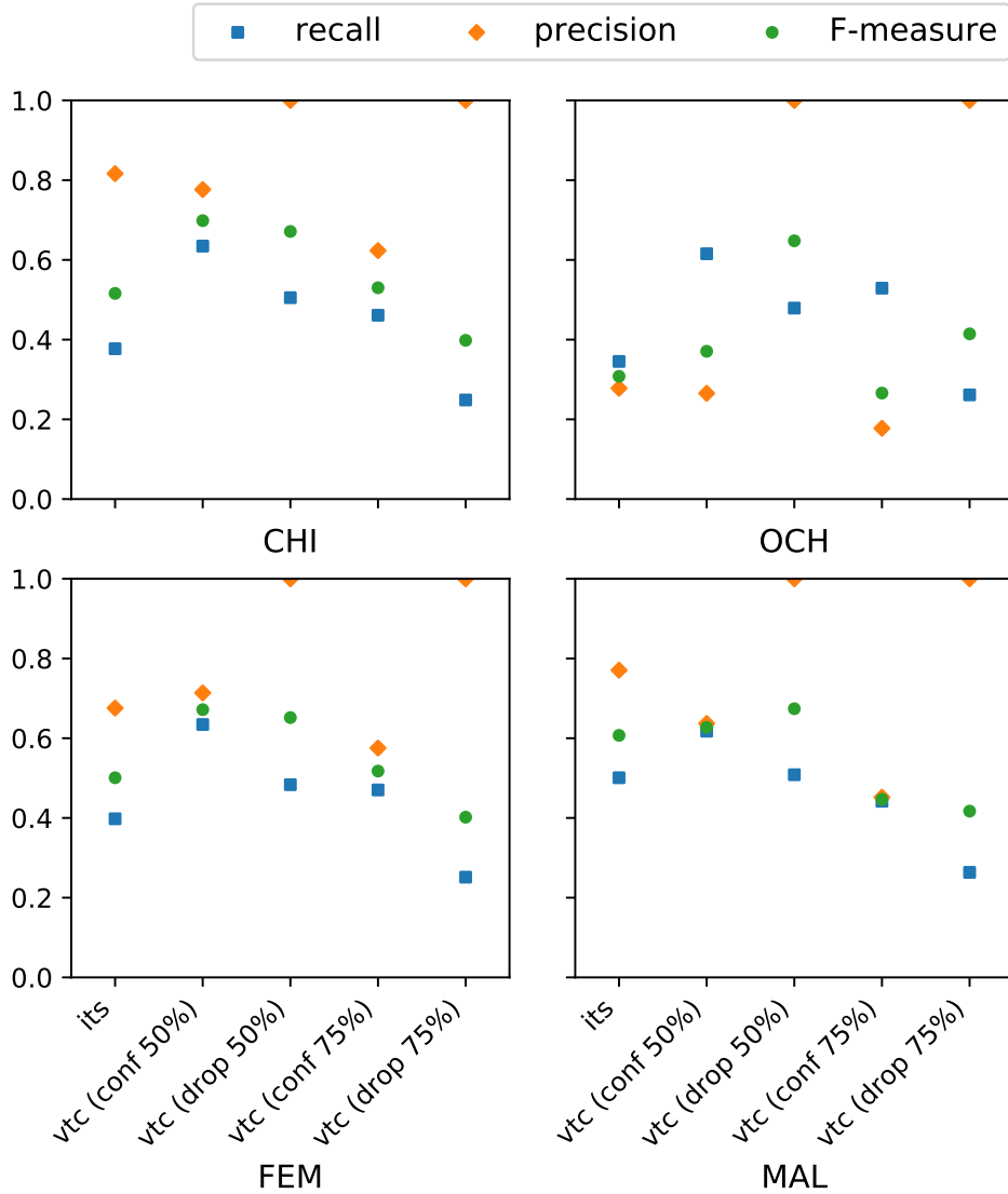
Fig. 4: Examples of diarization performance evaluation using recall, precision and F1 score. Audio from the the public VanDam corpus (VanDam, 2015) is annotated according to who-speak-when, using both the LENA diarizer (its) and the Voice Type Classifier (VTC) by Lavechin et al. (2020). Speech segments are classified among four speaker types: the key child (CHI), other children (OCH), male adults (MAL) and female adults (FEM). For illustration purposes, fake annotations are generated from that of the VTC. Two are computed by randomly assigning the speaker type to 50% and 75% (conf) of the VTC’s speech segments. Two are computed by dropping 50% of speech segments from the VTC (drop). Recall, precision and F1 score are calculated for each of these annotations, by comparing them to the VTC. The worst F-score for the LENA is reached for OCH segments. Dropping segments does not alter precision; however, as expected, it has a substantially negative impact on recall.
