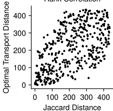
Rank Correlation
