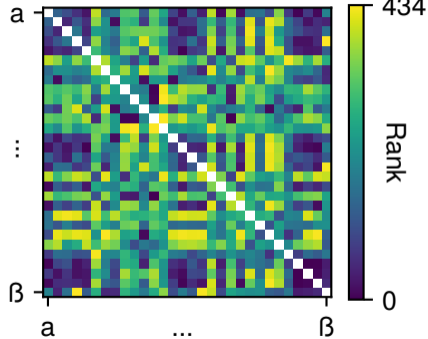
Wasserstein Distance
