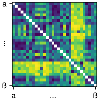
Jaccard Distance
