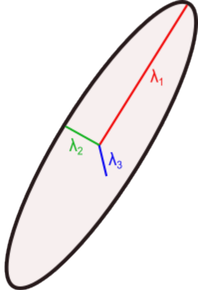
Anisotropic tensor
