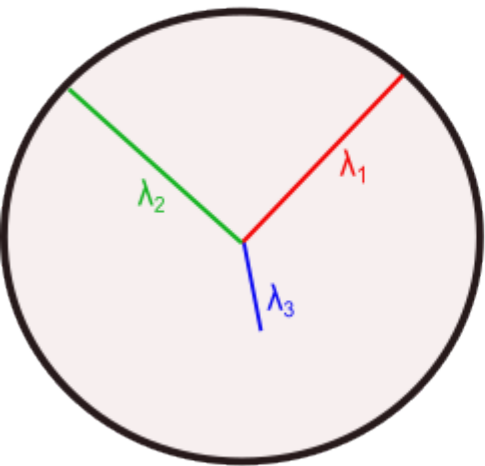
Isotropic tensor
